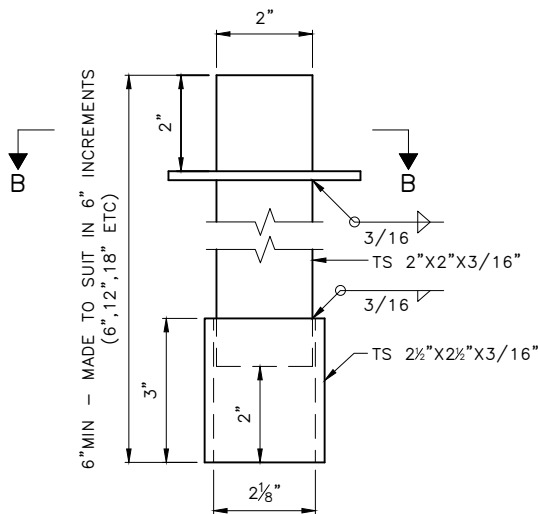
OPERATING NUT EXTENSION DETAIL
