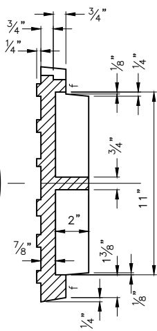
SECTION C-C
