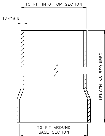
EXTENSION PIECE
