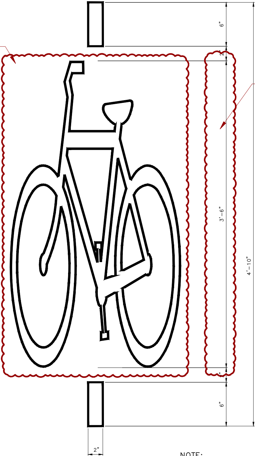
772 BICYCLE DETECTOR SYMBOL
