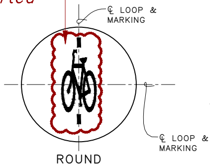
BICYCLE QUADRIPOLE
