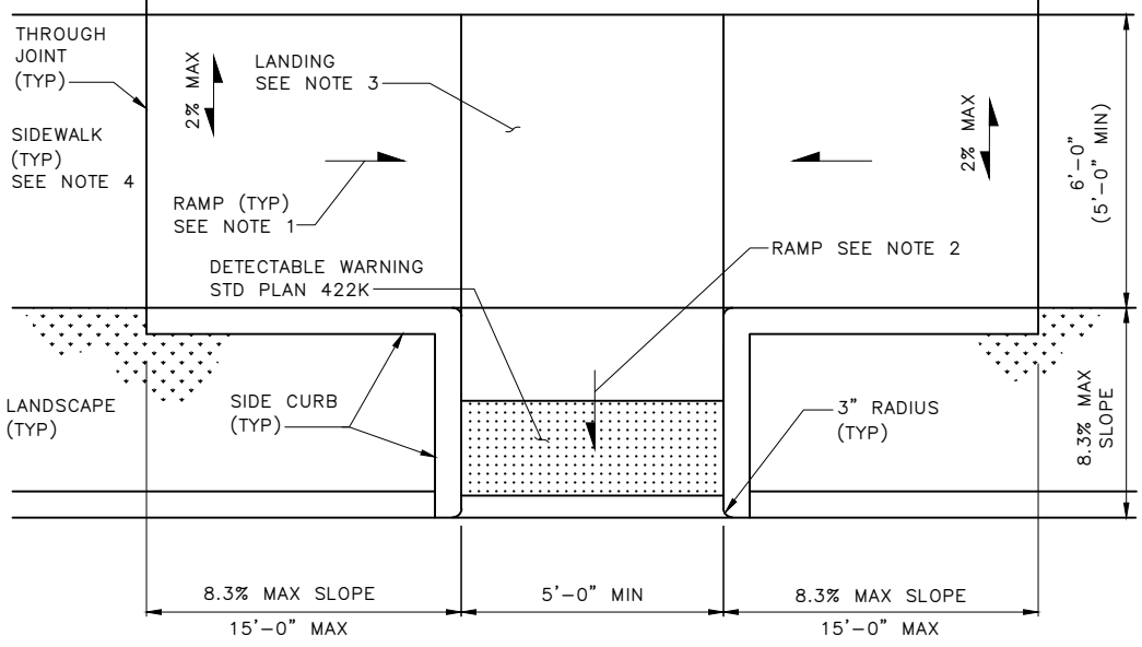
PARALLEL CURB RAMPS (TYPE 422B)
