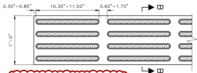
title changed — TACTILE DIRECTIONAL INDICATOR — CAST-IN-PLACE
