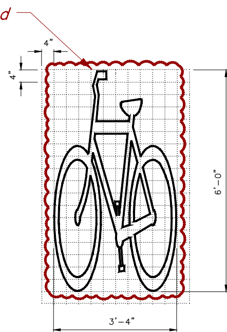
770C BIKE SYMBOL
