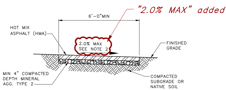
HOT MIX ASPHALT PAVEMENT SIDEWALK SECTION
