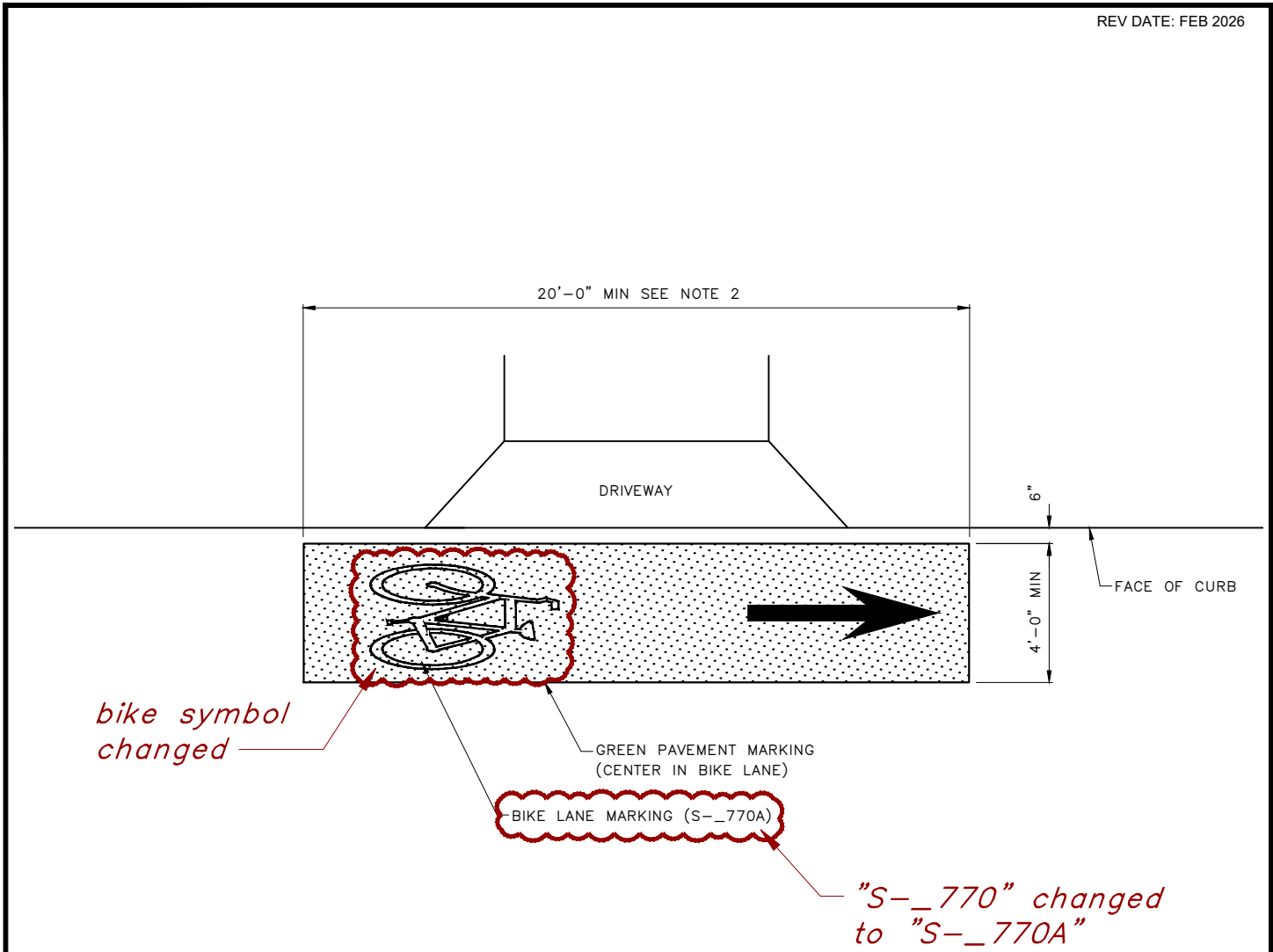
DRIVEWAY CROSSING LAYOUT
