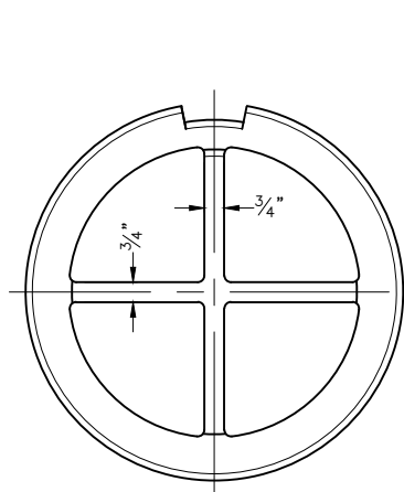
BOTTOM VIEW
