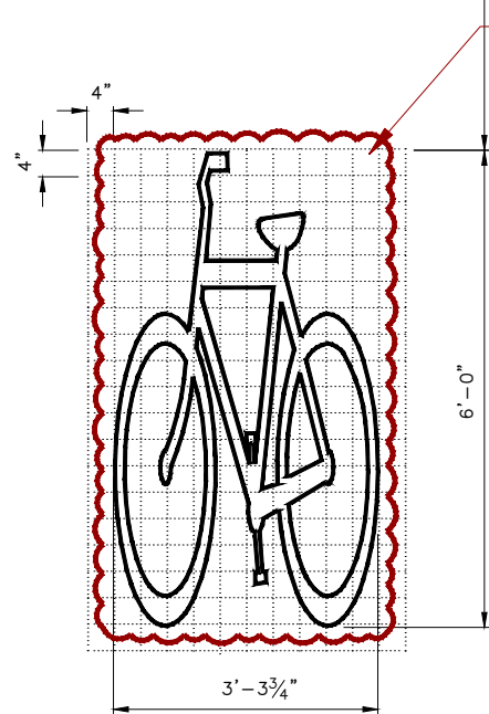
770A BIKE SYMBOL WITH ARROW
