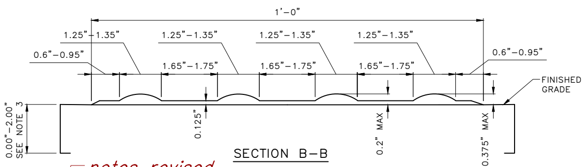
title changed — TACTILE DIRECTIONAL INDICATOR — CAST-IN-PLACE
