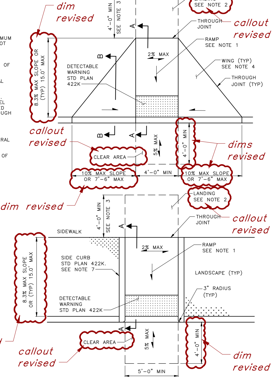
PERPENDICULAR CURB RAMPS (TYPE 422A)
