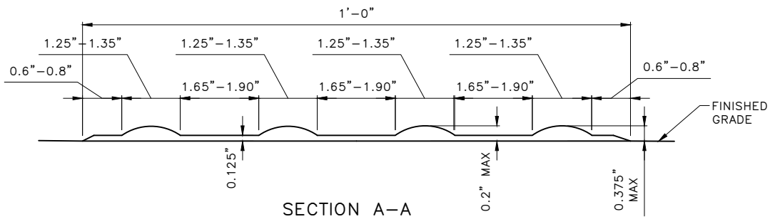
title changed — TACTILE DIRECTIONAL INDICATOR — SURFACE APPLIED
