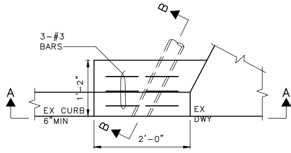
DRAIN DISCHARGE AT CURB FACE – PLAN VIEW
