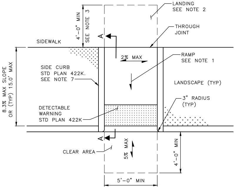
PERPENDICULAR CURB RAMPS (TYPE 422A)
