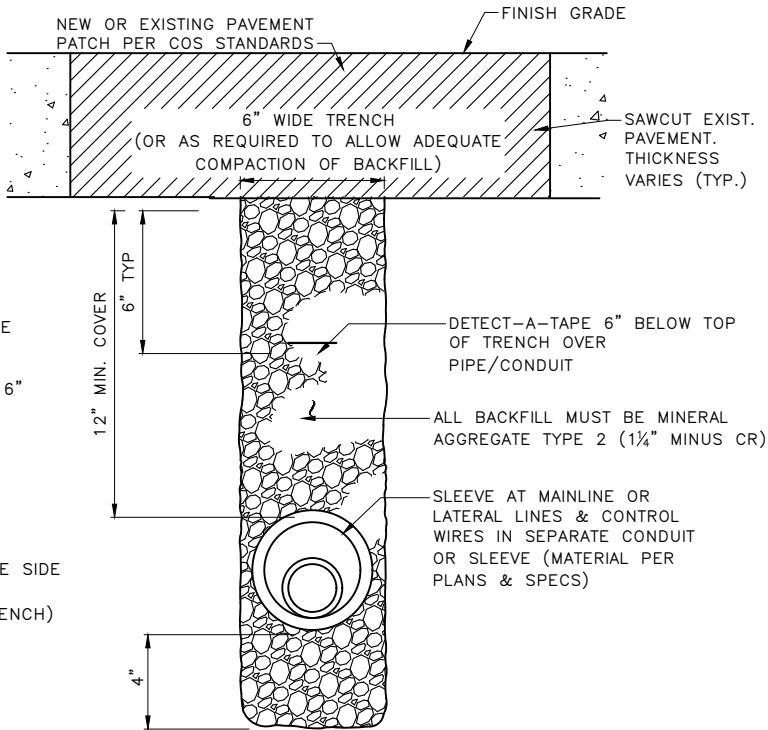
IRRIGATION SLEEVE TRENCHING UNDER PATHWAY OR SIDEWALK
