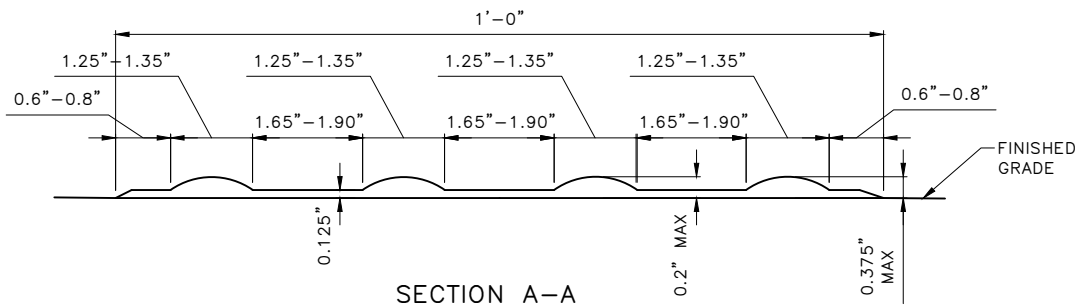
TACTILE DIRECTIONAL INDICATOR – SURFACE APPLIED
