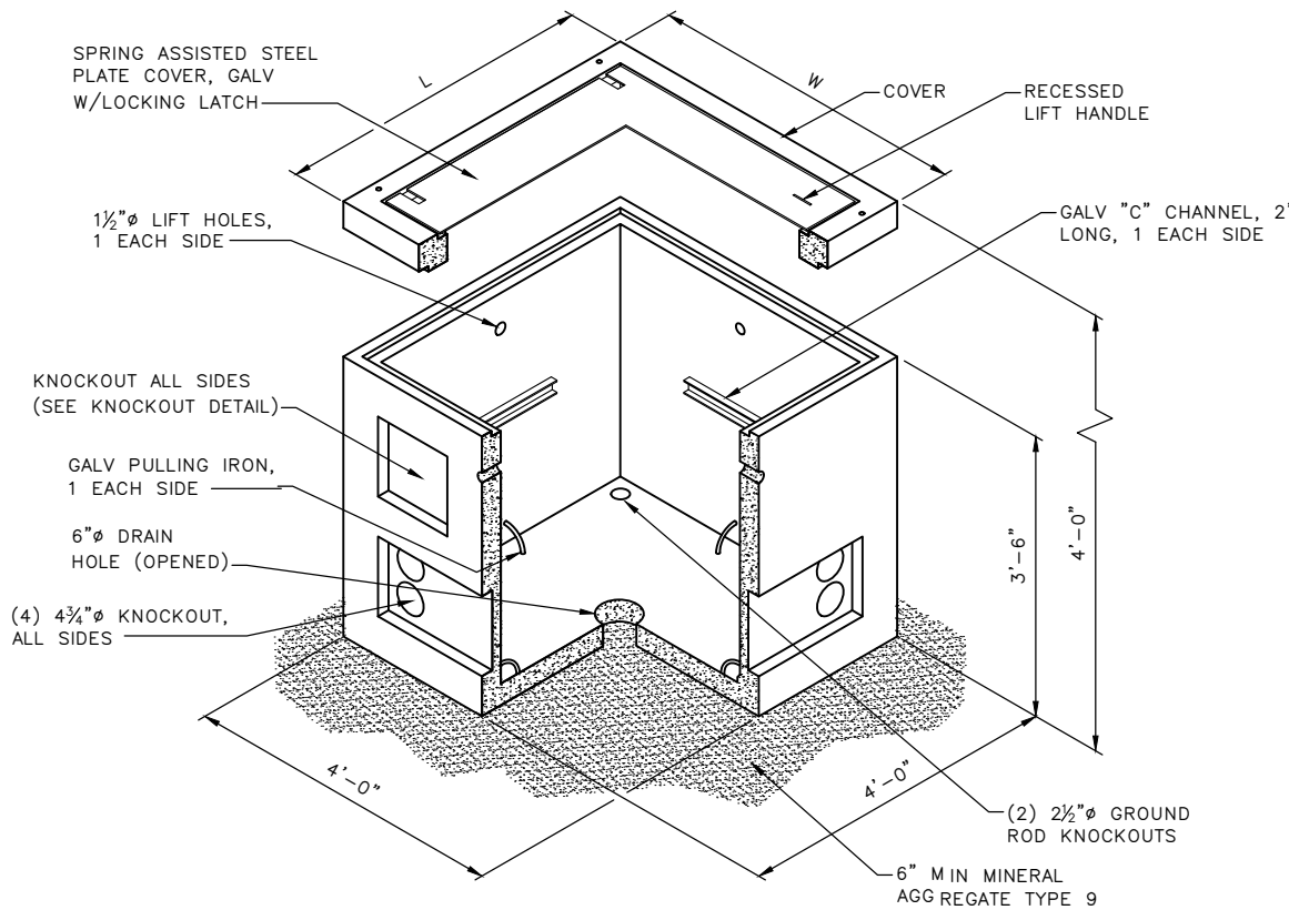
TYPE 6 HANDHOLE
