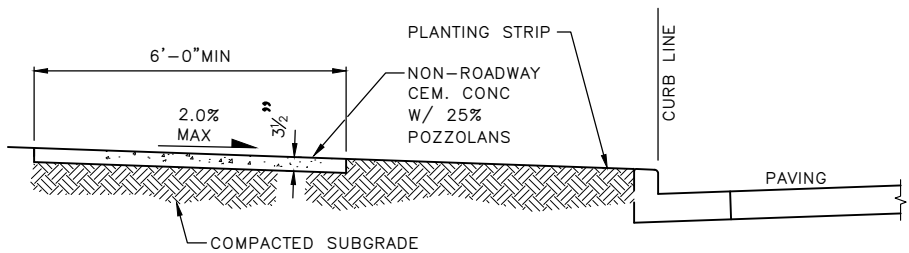
SECTION B-B
