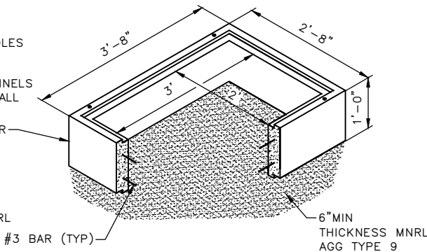
TYPE 3 HANDHOLE (COVER SAME AS TYPE 5)
