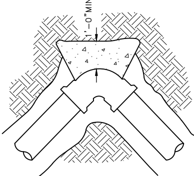
HORIZONTAL BEND
