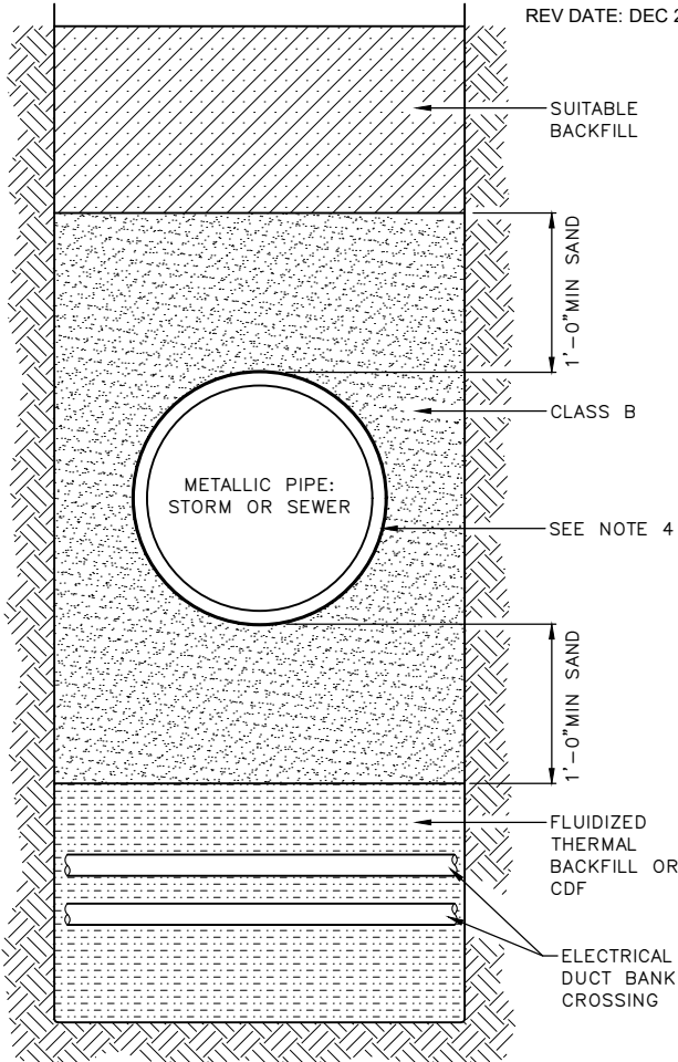
SAND BEDDING AT TRENCH CROSSING OF METAL PIPE
