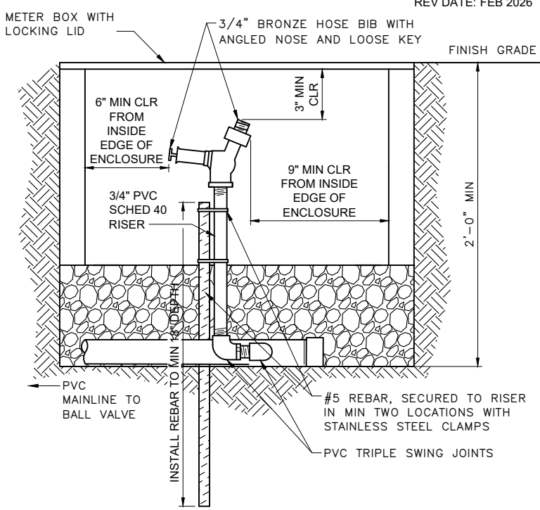
BELOW GROUND HOSE BIB
