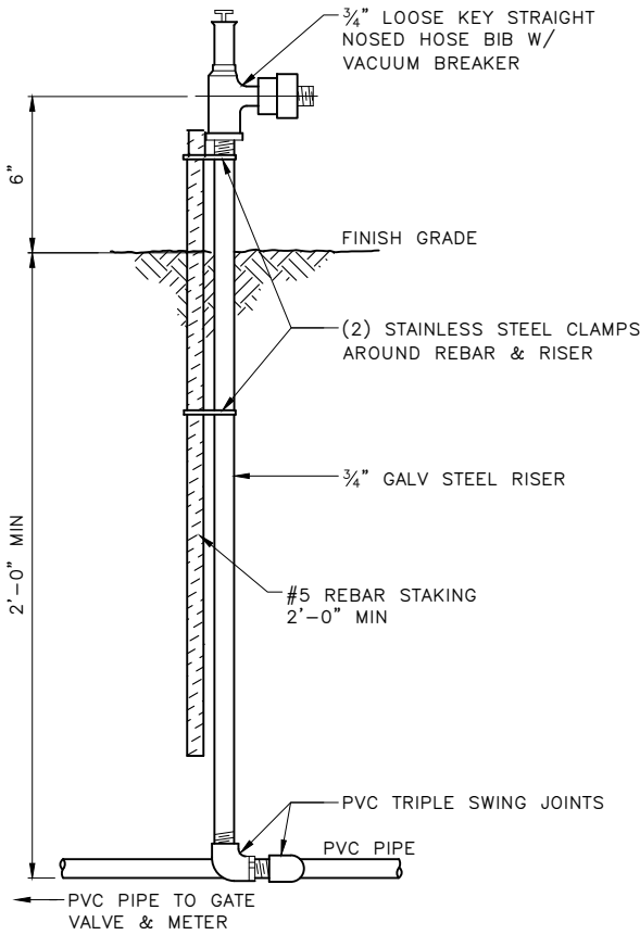
ABOVE GROUND HOSE BIB
