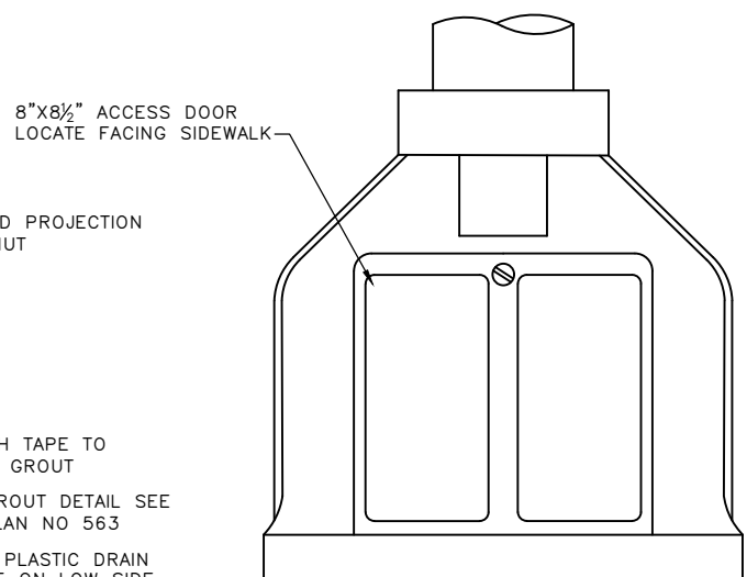
SQUARE BASE PEDESTAL
