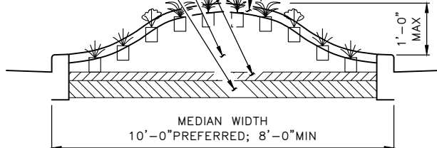
SOIL PREPARATION DETAIL
