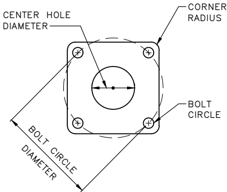
ANCHOR PLATE
