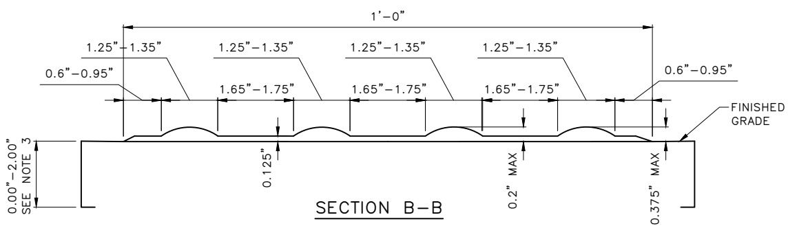
TACTILE DIRECTIONAL INDICATOR – CAST-IN-PLACE
