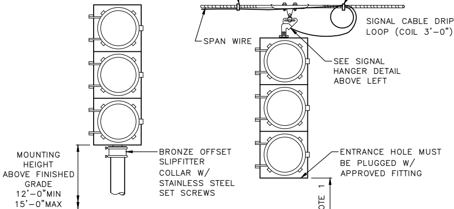
PEDESTAL TOP MOUNTING
