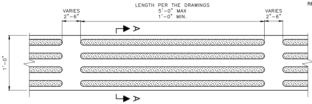
TACTILE DIRECTIONAL INDICATOR – SURFACE APPLIED
