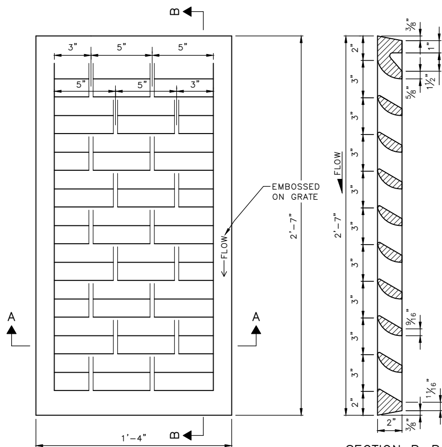
SECTION B-B
