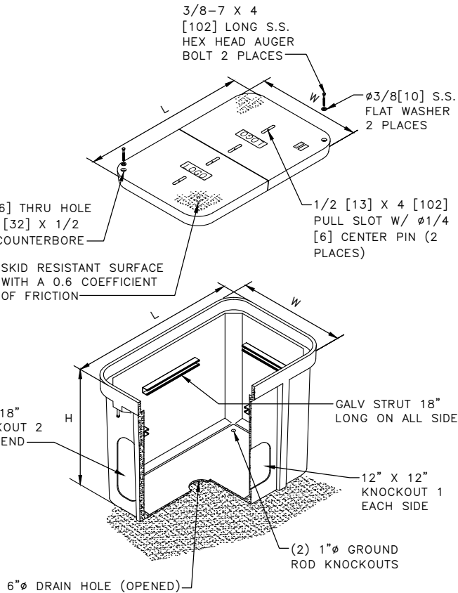
TYPE 5 HANDHOLE
