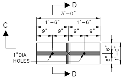
CURB PLAN
