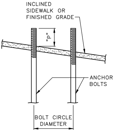
INCLINED CONDITION
