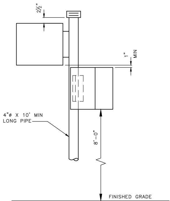
PEDESTAL MOUNT
