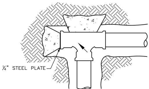
PLUGGED TEE
