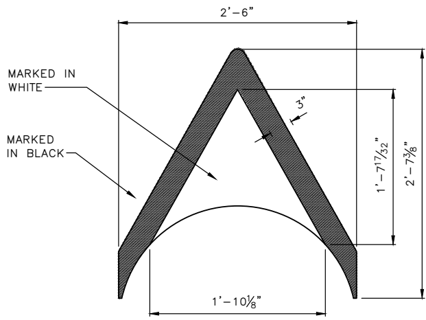
773B BIKE DOT ARROW
