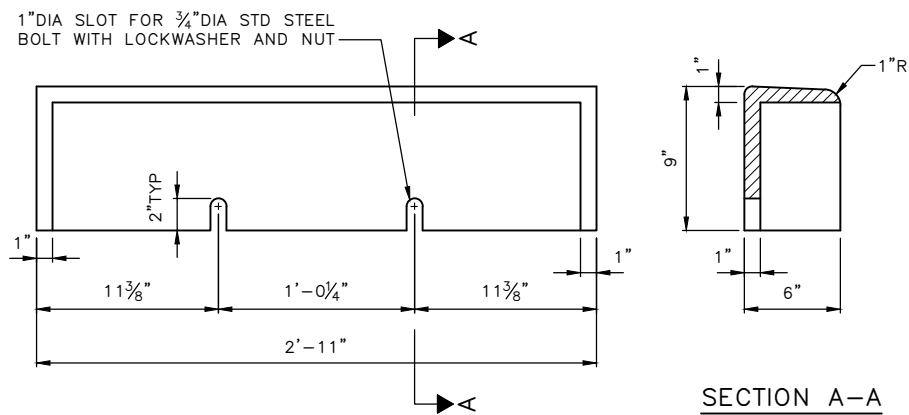
CURB INLET
