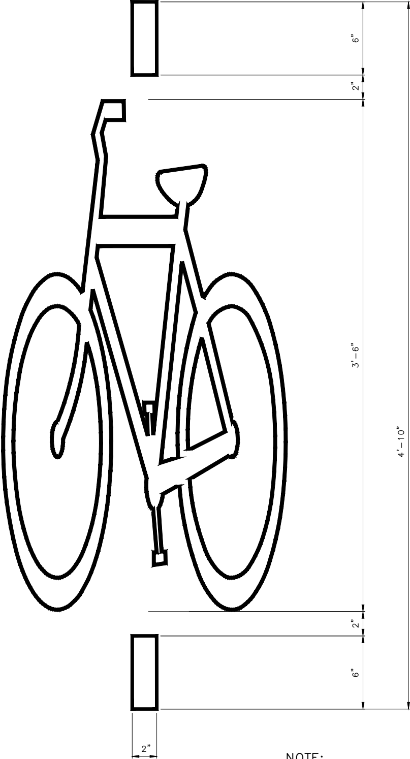
772 BICYCLE DETECTOR SYMBOL
