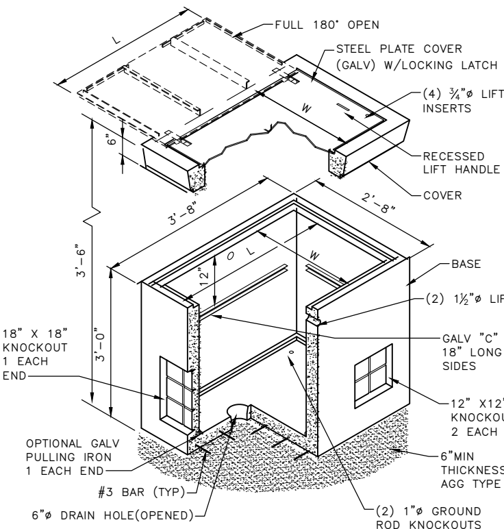
TYPE 5 HANDHOLE
