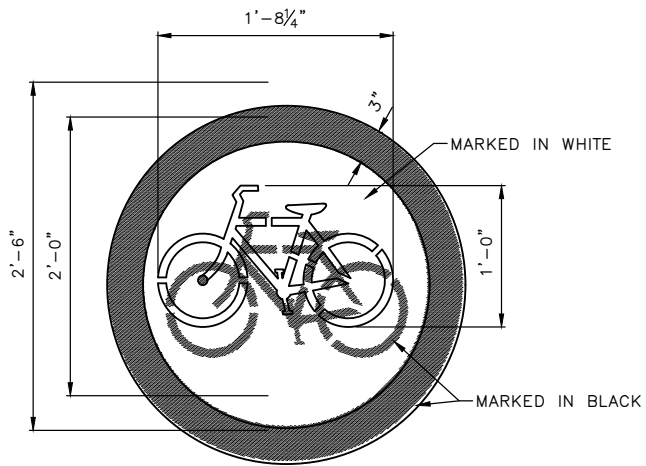
773C BIKE DOT SYMBOL
