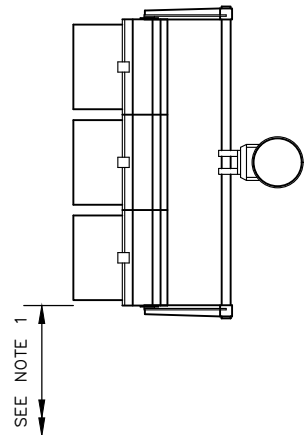
BRACKET MOUNTING FOR MAST ARM MOUNTED
