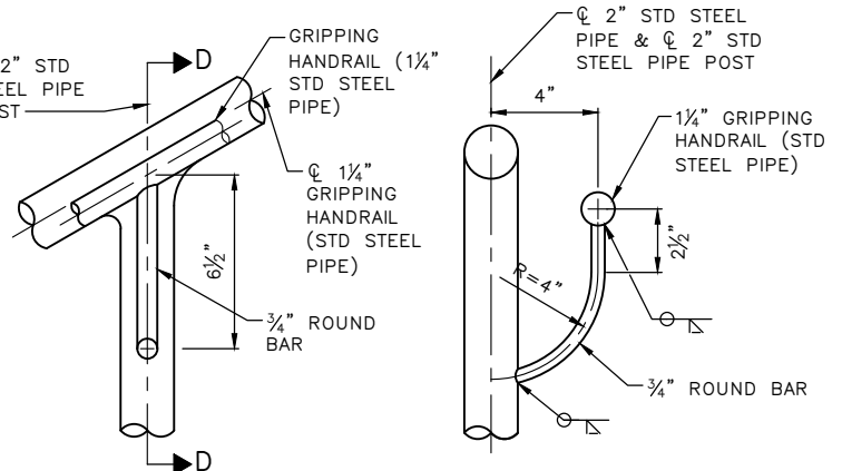
DETAIL D
