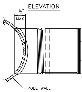
CABLE OUTLET DETAIL
