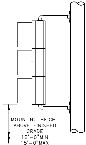
BRACKET MOUNTING FOR POLE MOUNTED
