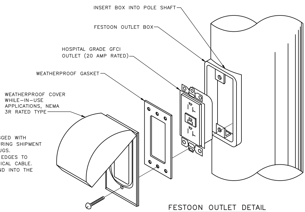
FESTOON OUTLET BOX
