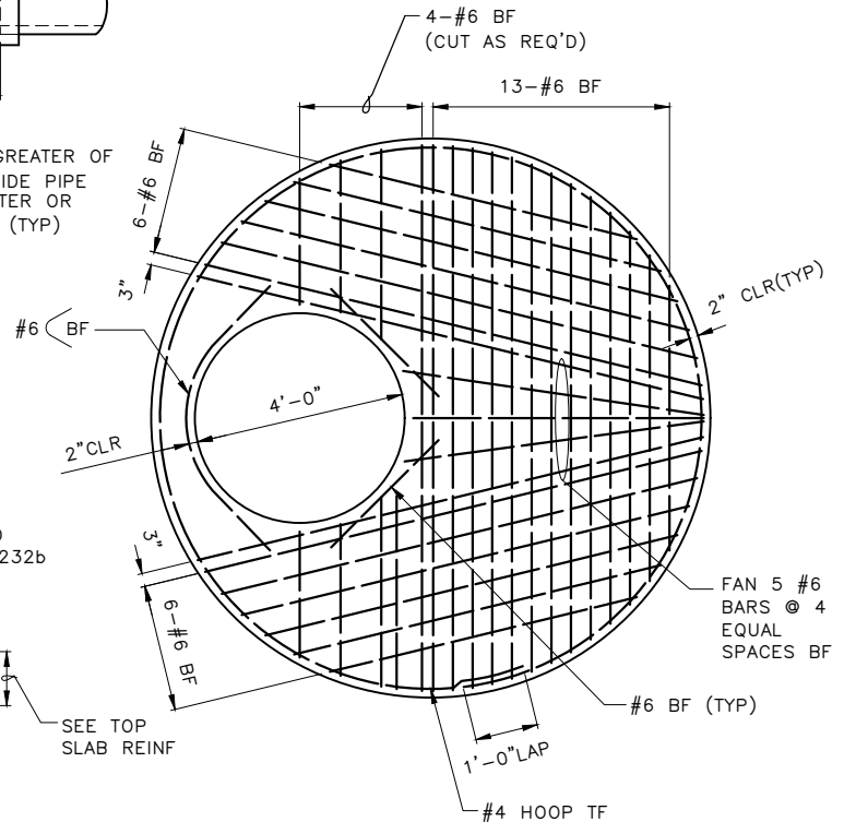
TOP SLAB REINFORCEMENT
