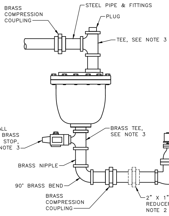
VALVE ASSEMBLY DETAIL
