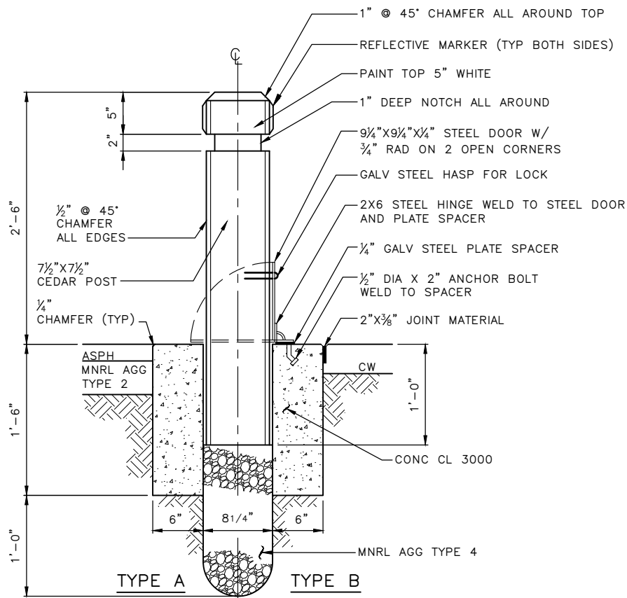
REMOVABLE BOLLARDS
