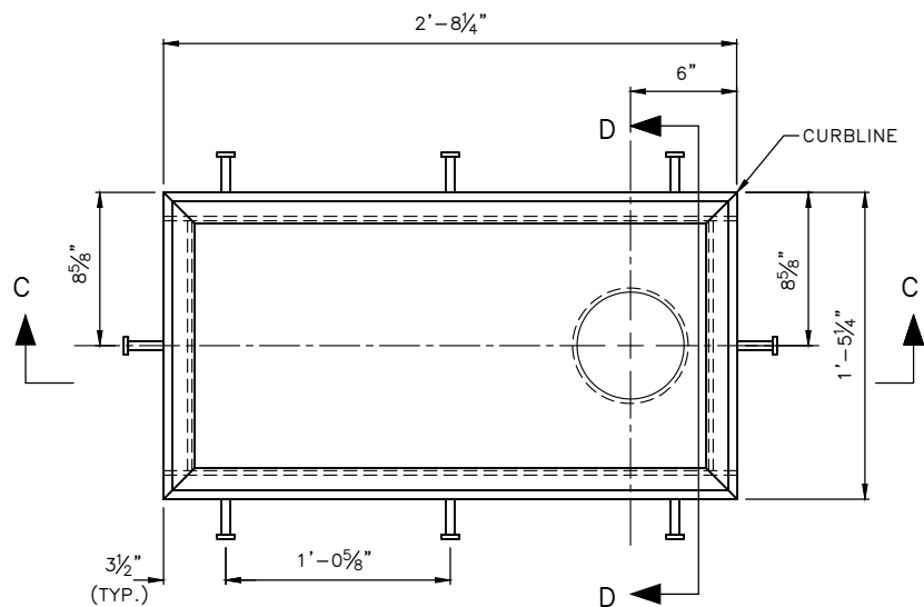
PLAN VIEW – BRIDGE DRAIN
