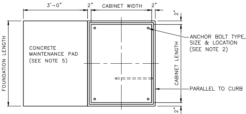
SIGNAL CONTROLLER FOUNDATION SEE STD PLANS NO 500b & 500c FOR CONDUIT LAYOUT
