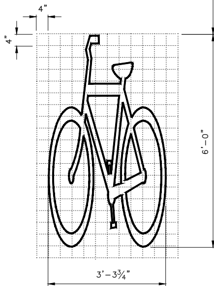
770A BIKE SYMBOL WITH ARROW
