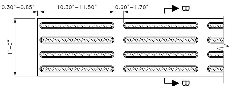
TACTILE DIRECTIONAL INDICATOR – CAST-IN-PLACE
