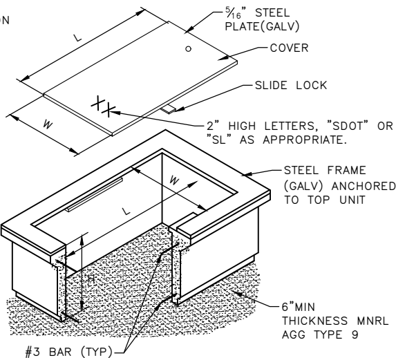
TYPE 1 & 2 HANDHOLE
