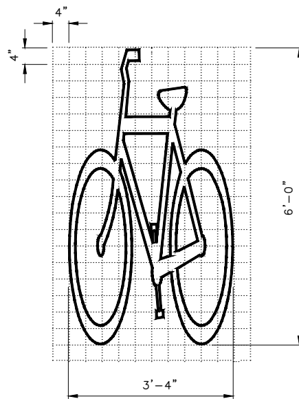
770C BIKE SYMBOL
