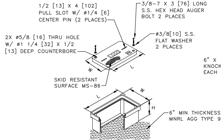
TYPE 1 & 2 HANDHOLE
